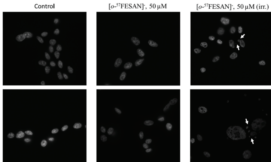
Fig. 11 Fluorescence microscopy for visualizing cellular responses in non-treated cells (control; left panel), or 50 \mu\text{M} \text{Na}[o\text{-}^{57}\text{FESAN}] -treated but non-irradiated cell (middle panel), or 50 \mu\text{M} \text{Na}[o\text{-}^{57}\text{FESAN}] -treated cells that were also subjected to Mössbauer irradiation (right panel). Morphological damage to the nucleus was observed as indicated by the presence of nuclear fragments and abnormalities (white arrows).
