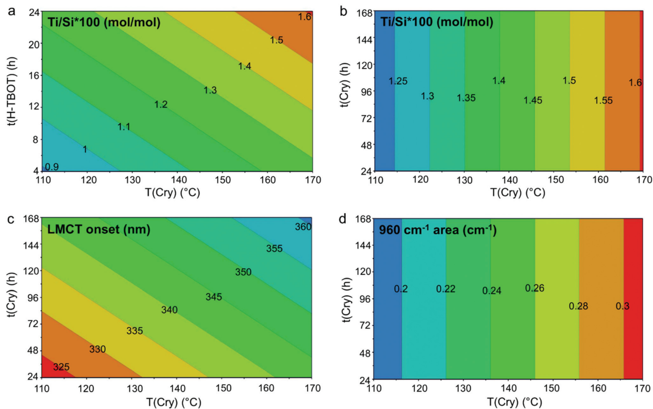
Fig. 3 Contour plots for the responses regarding Ti content (Ti/Si \times 100 in panels a and b) and speciation (LMCT onset in panel c and 960 cm -1 area in panel d). Panels a and c report the contour plots involving the significant variables for the responses Ti/Si \times 100 and LMCT onset, while panels b is included to compare the total Ti content with the LMCT onset and the 960 cm -1 area varying the same variables (time and temperature of crystallization). The askew bands are iso-response regions, delimited by lines which corresponding response is reported in the labels (the label have the dimension of the response).
