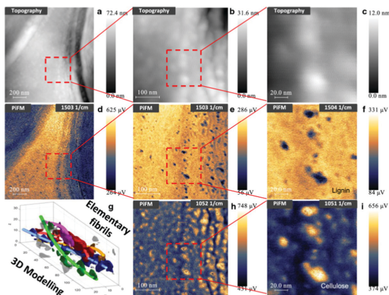
Fig. 10 Topography (a–c) and PiFM images (d–i) of an ultrathin Norway spruce cross-section at ca. 1503 (d–f) and 1052 (h and i) \text{cm}^{-1} at three different magnifications (dimensions shown by the scalebars). A TEM tomography image of a helical cellulose elementary fibrils (EF) bundle with its dimensions (nm) is also shown (g) (Reza et al. 57 ). The vertical cellulose-rich patterns in the PiFM images at ca. 1050\text{ cm}^{-1} may represent tangentially organized EF bundles that are typical of the S_1 layer of Norway spruce tracheids. Reproduced from Kesari et al. 56
