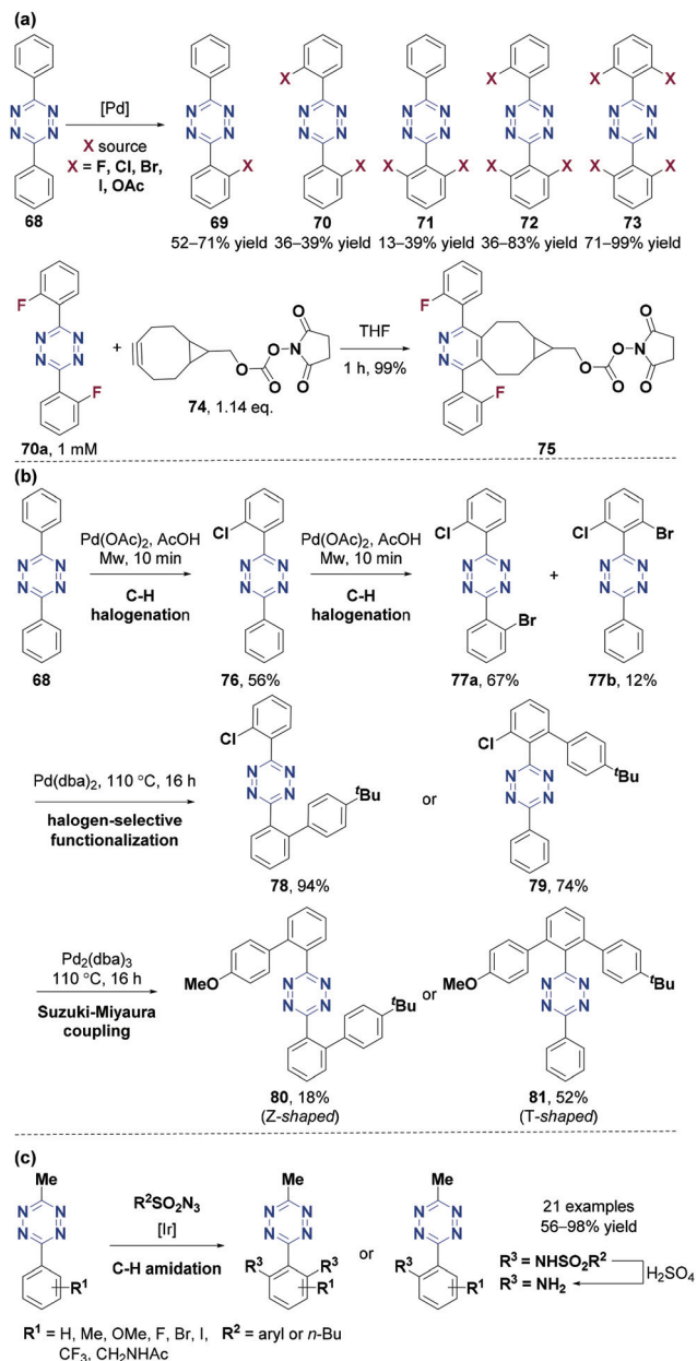
Fig. 9 Functionalization of aryl-substituted tetrazines via C–H activation. (a) ortho -Functionalized aryltetrazines prepared via direct Pd-catalyzed C–H activation/halogenation. (b) Synthesis of unsymmetrical polyhalogenated and biphenyl aryltetrazines via sequenced selective halogenation and Suzuki–Miyaura coupling reactions. (c) ortho -Functionalized aryltetrazines prepared via iridium-catalyzed C–H amidation.
