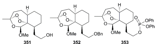
Fig. 17 Examples of peroxy bridge-containing artemisinin analogs.
