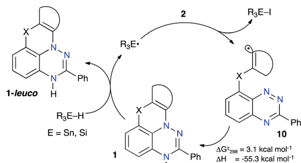
Fig. 3 Proposed mechanism for the formation of 1-leuco in a radical chain process and DFT-derived thermochemical parameters for the N-addition step in 10-a .
