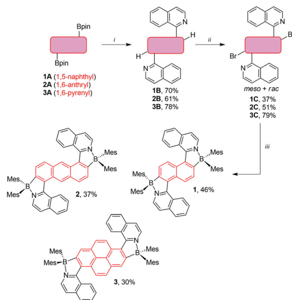
Scheme 2 Synthesis of the dyes 1–3 . (i) 2.6 equiv. 1-chloroisoquinoline, 6 mol% [Pd(PPh_3)_4] , toluene : MeOH (2 : 1), Na_2CO_3 (aq.), 90 °C. (ii) (1) 2.8 equiv. B_2pin_2 , 4 mol% [Ir(\mu-OMe)(cod)]_2 , 8 mol% 2-pyridinecarboxaldehyde N,N -dibenzylhydrazone, 1,4-dioxane, 90–100 °C. (2) 6.0 equiv. CuBr_2 , i -PrOH : MeOH (2 : 3), water, 90 °C. (iii) (1) 2.4 equiv. n -BuLi, anhydrous THF, –78 °C. (2) 3.0 equiv. Mes_2BF ( Mes : mesityl), –78 °C → rt.
