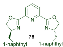
Scheme 57 La(III)-complexes in the conjugate addition of nitroalkanes to enones.
