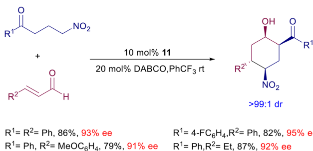
Scheme 13 Tandem conjugate addition/aldol reactions catalyzed by chiral prolinol 11 .
