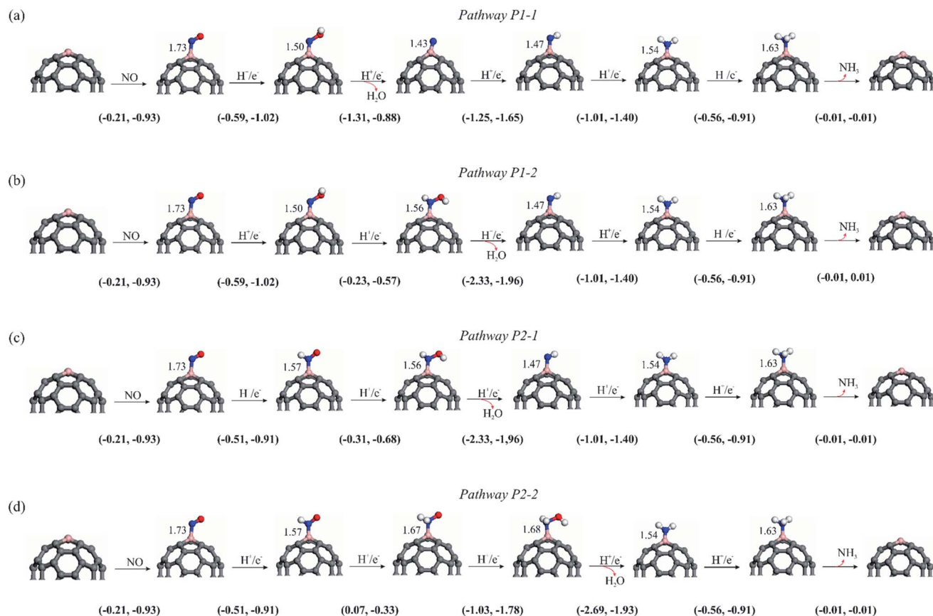
Fig. 5 Optimized structure of various intermediates for NOER to NH 3 along the (a) P1-1, (b) P1-2, (c) P2-1 and (d) P2-2 pathways over C 59 B. All B–N bond distances are in Å. The first number in the parentheses is the ΔG, while the second is the ΔE.
