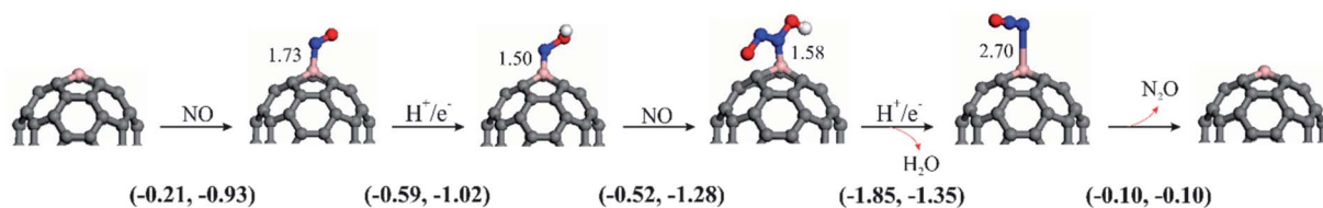
Fig. 6 Optimized structures of NOER species over C 59 B at high NO coverage. All B–N bond distances are in Å. The first number in the parentheses is the ΔG, while the second is the ΔE.
