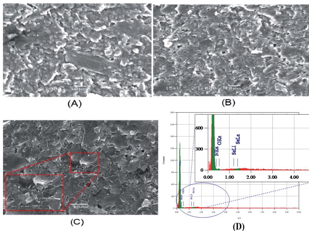
Fig. 4 SEM images of (A) p-AAQ/CPE, (B) p-AAQ/MWCNT/CPE and (C) p-AAQ/MWCNT/CPE after the deposition of 50 \mu\text{g L}^{-1} \text{Se}^{4+} for 60 s at -0.8 V, and (D) EDS of p-AAQ/MWCNT/CPE after the deposition of 50 \mu\text{g L}^{-1} \text{Se}^{4+} .
