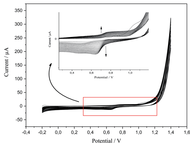
Fig. 1 CV of p-AAQ/CPE in 0.1 M HCl at a scan rate of 0.1 V s -1 for 20 scanning cycles.
