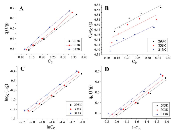
Fig. 4 Line of isothermal adsorption at different temperatures (A), linear plots of the Langmuir (B), Freundlich (C) and Temkin (D) models at different temperature.
