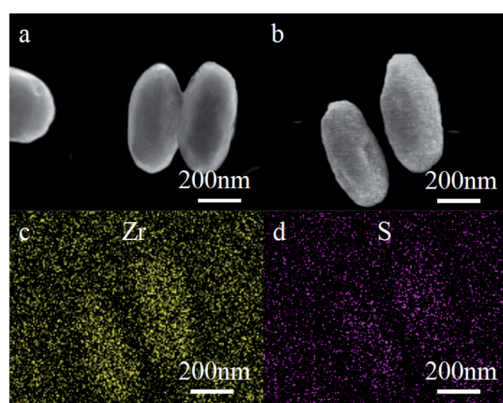
Fig. 4 SEM images of (a) PCN-222 and (b) L-Cys-PCN-222, and EDS patterns of (c) Zr and (d) S elements in L-Cys-PCN-222, respectively.
