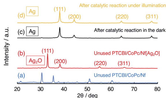
Fig. 2 XRD patterns of (a) PTCBI/CoPc-Nf, (b) unused PTCBI/CoPc-Nf [Ag 2 O], and (c) PTCBI/CoPc-Nf [Ag 2 O] after the N 2 H 4 oxidation (c) in the dark and (d) under irradiation.
