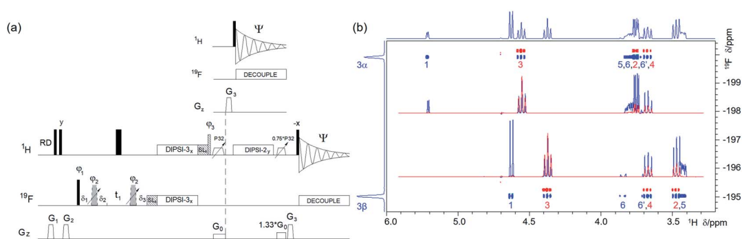
Fig. 4 (a) Pulse sequence of a 2D ^{19}\text{F} , ^1\text{H} CP-DIPSII3–DIPSII2. For explanation of symbols used for pulses see Experimental. The NMR parameters used are given in Table S1.† The dashed line indicates signal acquisition before an optional ^1\text{H} – ^1\text{H} spin-lock. For description of pulses see Experimental. The delays were as follows: \delta_1 = 20 \mu\text{s} ; \delta_2 = \delta_1 + (2/\pi) \times p3 ; \delta_3 = p2 ; t_1(0) is the initial t_1 evolution delay time = 0.5 \times \text{in}0 , where \text{in}0 is the t_1 increment. The gradient strengths were as follows: G_0 = 5\% ; G_1 = 17\% ; G_2 = 31\% ; G_3 = 66\% . The following phase cycling was used: \varphi_1 = y, -y ; \varphi_2 = 4x, 4(-x) ; \varphi_3 = 2y, 2(-y) ; \Psi = x, 2(-x), x . The states-TPPI protocol was used for sign discrimination in F_1 with the phase \varphi_1 incremented by 90^\circ . Purging of ^{19}\text{F} magnetisation at the beginning of the pulse sequence by a composite 90^\circ ^{19}\text{F} pulse and PFGs minimises the cancellation artefacts. (b) An overlay of two 2D ^{19}\text{F} , ^1\text{H} CP-DIPSII3–DIPSII2 spectra acquired with 20 ms ^{19}\text{F} \rightarrow ^1\text{H} cross-polarisation (CP) only (red) and an additional 50 ms ^1\text{H} \rightarrow ^1\text{H} spin-lock (blue) using the pulse sequence shown in (a). The red spectrum was offset vertically to facilitate visualisation of the cross peaks. The two insets show overlaid 1D F2 traces through ^{19}\text{F} resonances of \alpha - and \beta -D-glucose from both spectra. Twice as many scans were acquired for the blue spectrum as for the red spectrum. 1D ^{19}\text{F} and ^1\text{H} projections of the blue spectrum are shown along the left and top, respectively.
