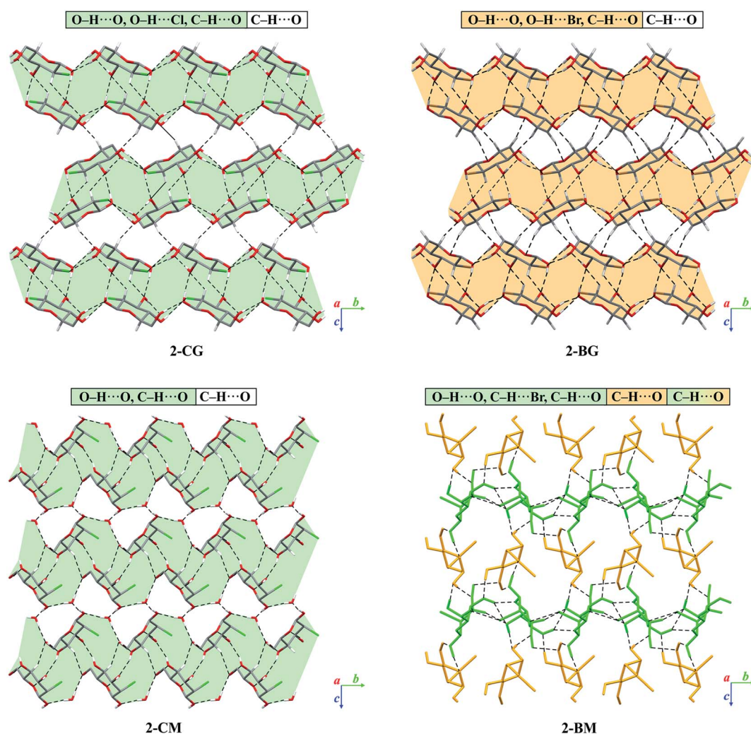
Fig. 4 Comparison of packing of molecules in the crystals of brominated derivatives of 2-DG with their chlorinated counterparts. The dashed lines represent hydrogen bonds. The H-atoms not participating in intermolecular hydrogen bonds have been omitted for the sake of clarity. Layered supramolecular entities in 2-CG , 2-CM and 2-BG have been highlighted in either light-orange (bromine) or light-green (chlorine). Different anomers of 2-BM were depicted as orange ( \alpha -anomer, layer A) or green ( \beta -anomer, layer B).
