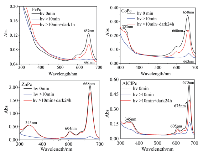
Fig. 2 UV-vis spectra of photo-excited and dark-treated FePc, CoPc, ZnPc and AlClPc in DMF.
