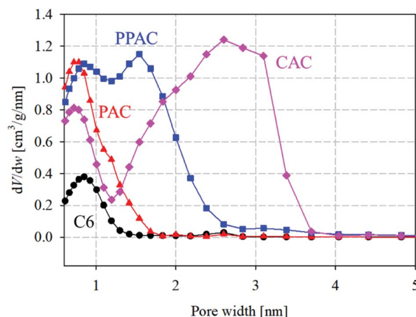
Fig. 2 Pore size distributions for starting carbonized material and derived activated carbons (circle) C6; (triangle) PAC; (square) PPAC; (diamond) CAC.
