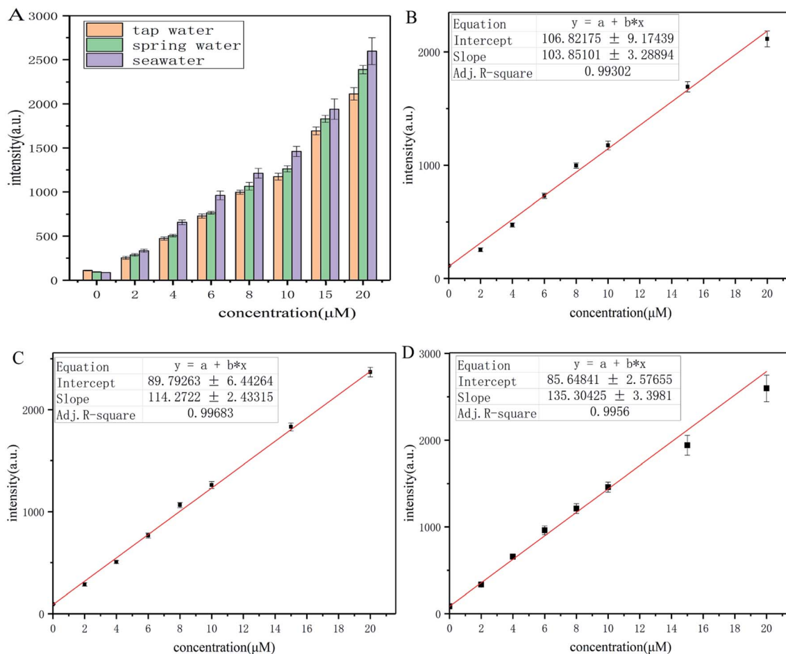
Fig. 6 (A) Fluorescence response of probe-dbp (5 \mu\text{M} ) towards various concentration of p -thiocresol in different water samples, including tap water, spring water and seawater. The linear relationship between the fluorescence intensity of probe-dbp at 570 nm and the concentration of p -thiocresol in tap water (B), spring water (C) and seawater (D).
