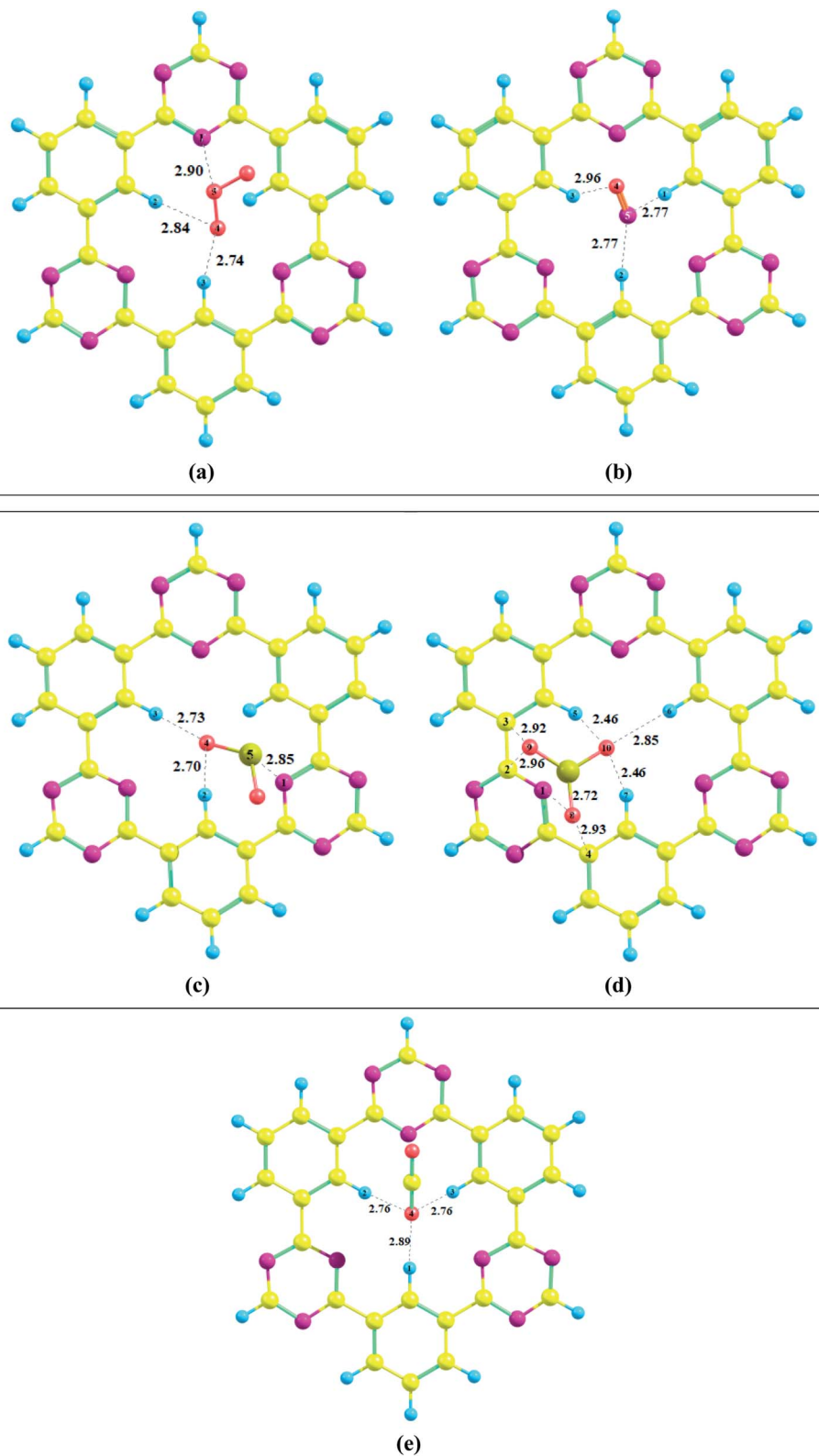
Fig. 2 Optimized geometries of selected analytes at CTF-0 surface (top view) at M05-2X/6-31G++(d,p) level of theory. In analytes, pink color indicates the presence of O-atom, mustard yellow presents S-atom, magenta color for N-atom, and yellow denotes C-atom. (a) O_3@CTF-0 , (b) NO@CTF-0 , (c) SO_2@CTF-0 , (d) SO_3@CTF-0 and (e) CO_2@CTF-0 .
