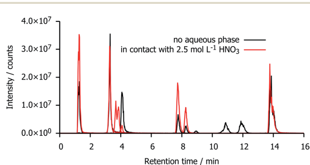
Fig. 5 Combined ion chromatograms of the most intense signals in irradiated mTDDGA samples with an initial concentration of 0.05 mol L -1 mTDDGA irradiated with or without contact to an aqueous phase of 2.5 mol L -1 HNO 3 .
