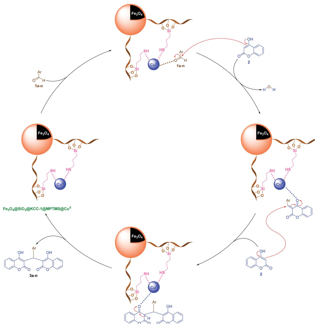
Scheme 5 Plausible mechanism for the solvent-free one-pot pseudo -three-component synthesis of bis-coumarins (3a–n) catalyzed by the \text{Fe}_3\text{O}_4@\text{SiO}_2@\text{KCC-1}@\text{MPTMS}@\text{Cu}^{\text{II}} nanocomposite.
