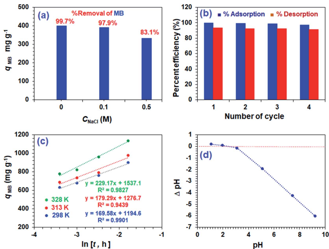
Fig. 7 (a) MB adsorption capacity, q_e and percent removal in the presence of NaCl. [CPZA 7: (50 mg), 1000 ppm MB solution (20 mL)]; (b) percent efficiencies of adsorption/desorption over four cycles. [CPZA 7 (100 mg), 1000 ppm MB (40 mL), pH 7.25]; (c) plot of Elovich kinetic model [250 mg CPZA 7, 100 mL 3000 ppm MB, pH 7.25]; (d) determination of pH of point of zero charge.
