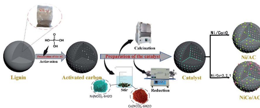
Scheme 1 Schematic illustration of the preparation of the \text{Ni}_x\text{Co}_y/\text{AC} catalyst.
