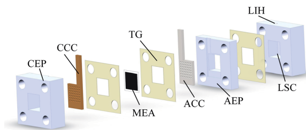
Fig. 1 Schematic diagram of \mu DMFC.
