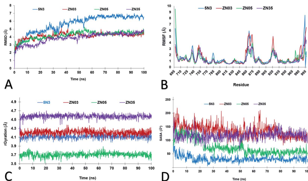
Fig. 4 Shows (A) RMSD of the protein backbone with respect to the first frame of MD simulation, (B) RMSF profile for C_{\alpha} atoms of protein residues, (C) radius of gyration plot as a function of simulation time for ligands only, (D) solvent accessible surface area for three lead molecules and co-crystallized ligand.
