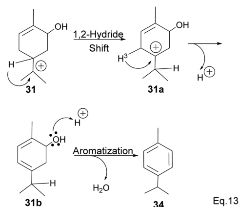
Scheme 10 Aromatization of terpenol to p -cymene.
