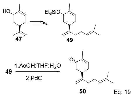
Scheme 15 Synthesis of cryptomerone 50 from \alpha -pinene allylic alcohol.
