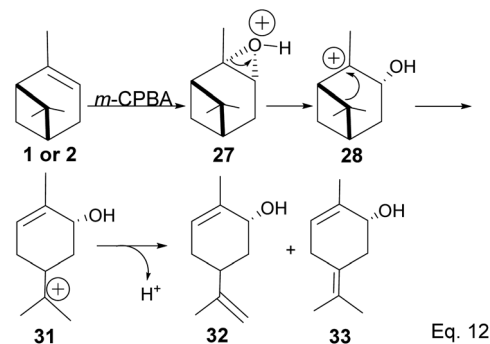
Scheme 9 Epoxide rearrangement via 1,2- \sigma -alkyl shift of pinene bridgehead to form terpenol derivatives.
