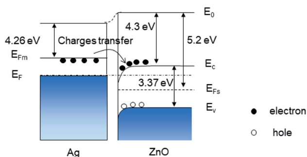
Scheme 2 Energy band diagram of ZnO/Ag interface showing the electron transfer between Ag and ZnO. 61
