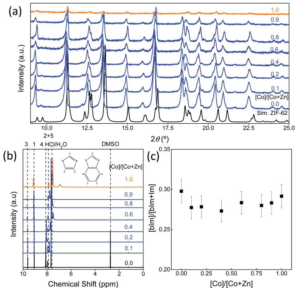
Fig. 2 (a) XRD patterns of the standard ZIF-62 series with varying the ratio of cobalt content to the total metal content ( [Co]/([Co + Zn]) ). (b) Liquid ^1H -NMR spectra of Co/Zn-ZIF-62 samples. Dashed lines: the typical peaks associated with imidazole, benzimidazole, and solvents. (c) Fraction of benzimidazole content in the total linker content for each cobalt modified ZIF-62, with a margin of error of 5%.
