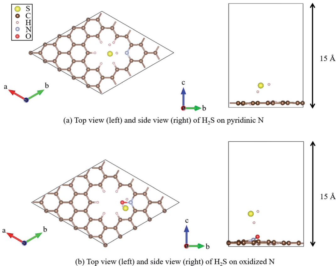
Fig. 2 Top and side views of the geometry optimized structure of H 2 S on (a) pyridinic N and (b) oxidized N.
