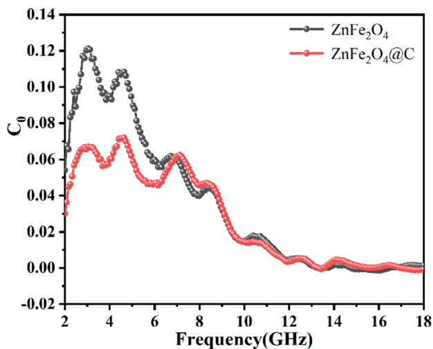
Fig. 11 C_0 values of \text{ZnFe}_2\text{O}_4 and \text{ZnFe}_2\text{O}_4@\text{C} .
