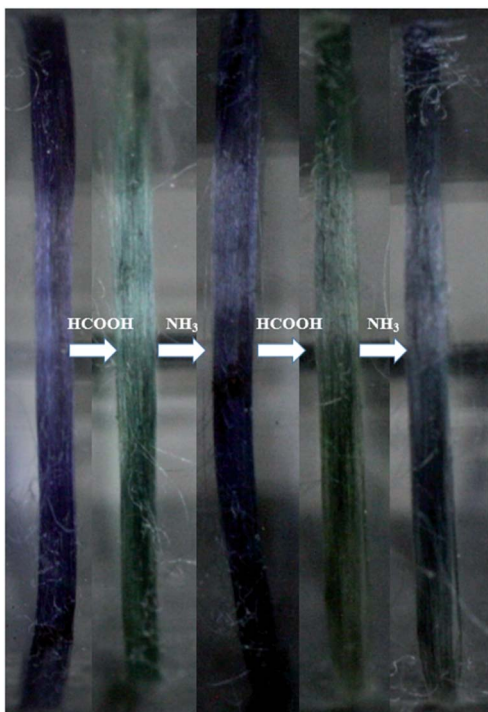
Fig. 6 Optical images of as-prepared aniline tetramer/dragline silk composite fibers cyclically exposed to formic acid (HCOOH) and ammonia ( \text{NH}_3 ) vapors. (Exposure time: HCOOH for 1 minute and \text{NH}_3 10 minutes, respectively) (dragline silk is modified with 1% of aniline tetramer solution).
