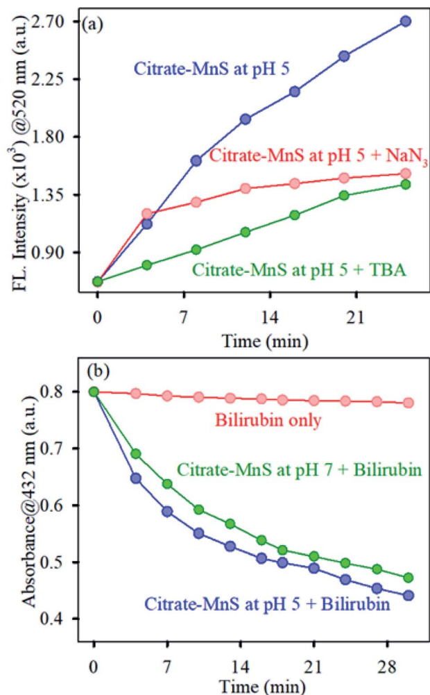
Fig. 4 (a) DCFH oxidation (monitored at 520 nm) with time in presence of citrate-MnS at pH 5 with singlet oxygen scavenger NaN 3 (red), hydroxyl radical scavenger (green) and without any scavenger (blue). (b) Bilirubin degradation by citrate-MnS at pH 5 (blue), pH 7 (green) and bilirubin only (red).
