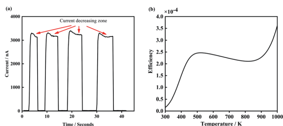
Fig. 9 (a) Is the I - t curve of GA irradiate by 5.5 W laser, (b) is the theoretical efficiency curve of the PETE devices.
