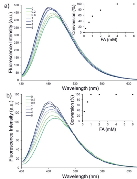
Fig. 3 Fluorescence response of (a) QA1 (10 \mu\text{M} ) and (b) QA2 (10 \mu\text{M} ) upon increasing concentrations of FA (0–6 mM) in \text{CH}_3\text{CN} -10 mM PBS buffer pH 7.4 (1 : 9, v/v) (contain 0.1% mouse serum) at 37 °C. Incubation time of QA1 and QA2 were 60 min and 15 min, respectively. \lambda_{\text{ex}} = 410 \text{ nm} .
