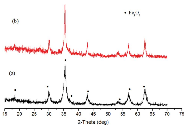
Fig. 7 XRD patterns of solid products after reduction of \text{Fe}(\text{NO}_3)_3 (a) and \text{FeCl}_3 (b) by glucose, respectively (250 °C, 3 h).
