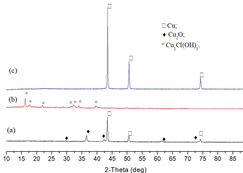
Fig. 6 XRD patterns of solid products after reactions of cellulose with \text{CuSO}_4 (a), \text{CuCl}_2 (b) and \text{Cu}(\text{NO}_3)_2 (c) (250 °C, 3 h).
