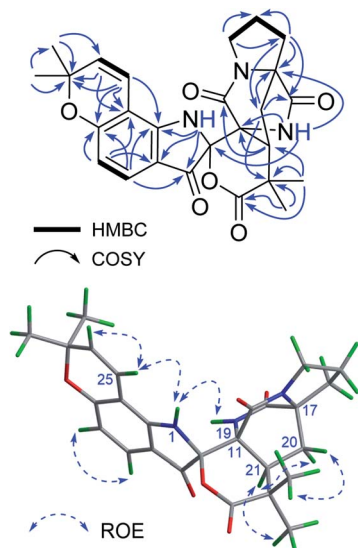
Fig. 2 Key HMBC, ^1\text{H} - ^1\text{H} COSY, and ROE correlations of 1 .
