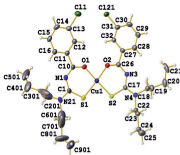
Fig. 21 Molecular structure of bis( N,N -di- n -butyl- N ',-3-chlorobenzoilthioureato) copper(II) complex 73d.
