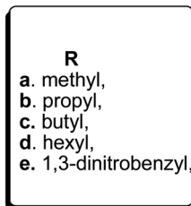
Scheme 37 Thioureas with different alkyl chains.
