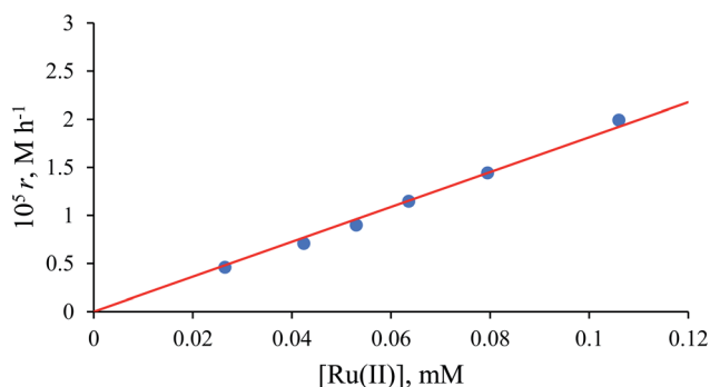
Fig. 10 Dependence of the initial rate on [\text{Ru}(\text{II})] for the catalysed reduction of \text{NAD}^+ to 1,4-NADH in water/ethanol (1 : 9, v/v) solution. Experimental conditions: [\text{NAD}^+] = 0.31 \text{ mM} , [\text{HCOO}^-] = 43.5 \text{ mM} , T = 36.8 \text{ }^\circ\text{C} .
