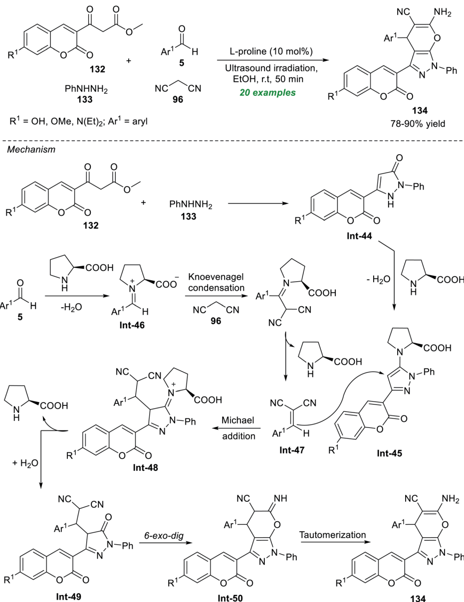
Scheme 37 Organocatalytic sonochemical synthesis of pyrano[2,3-c]pyrazoles linked with coumarin.
