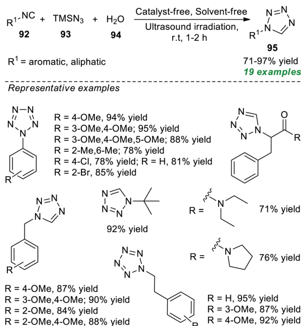
Scheme 24 Tetrazoles obtained by the ultrasound-assisted isocyanide-based multicomponent click reaction.
