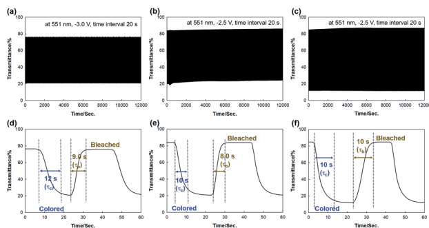
Fig. 3 Kinetic stability for [OHV-POSS][PF 6 ] 16 -based ECDs with ITO thicknesses of (a) 68.5 nm, (b) 140.3 nm, and (c) 252.1 nm during constant potential stepping between (coloration) and short-circuit (bleaching) conditions. The corresponding switching times required for coloration and bleaching of the ECDs are shown in (d)–(f). Resistance for faster electron movement. Moreover, it is also apparent that the OHV-POSS-based ion gel possessed high ionic conductivity, leading to a quicker charge transfer process.
