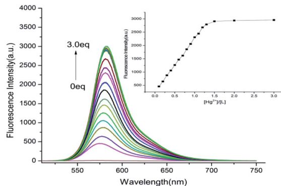
Fig. 4 Fluorescence emission spectra of probe L in the presence of various concentrations of \text{Hg}^{2+} (0–3 equiv.) in \text{CH}_3\text{OH}-\text{H}_2\text{O} (4 : 1, v/v, Tris-HCl buffer pH = 8.0).
