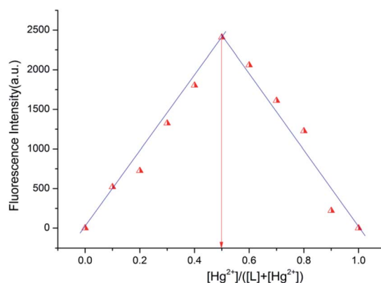
Fig. 5 Job's plot for determining the stoichiometry between L and \text{Hg}^{2+} ion in \text{CH}_3\text{OH}-\text{H}_2\text{O} (4 : 1, v/v, Tris-HCl buffer pH = 8.0).
