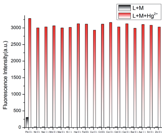
Fig. 3 The fluorescence intensity of L with \text{Hg}^{2+} in the presence of various competitive metal ions in \text{CH}_3\text{OH}-\text{H}_2\text{O} (4 : 1, v/v, Tris-HCl buffer pH = 8.0).
