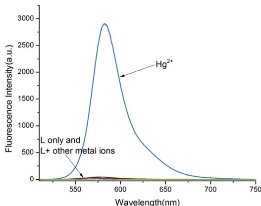
Fig. 2 Fluorescence responses of probe L upon treated with 10 equiv. metal ions in \text{CH}_3\text{OH}-\text{H}_2\text{O} (4 : 1, v/v, Tris-HCl buffer pH = 8.0).
