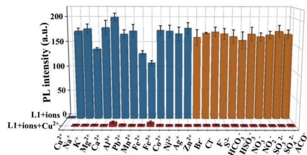
Fig. 5 Fluorescence intensity changes of L1 in the presence of Cu ^{2+} along with other cations and anions in the solution ( V_{water}/V_{THF} = 4/1 ). The concentration of L1 is 1 \times 10^{-5} mol L ^{-1} . The concentration of cation and anion are 1 \times 10^{-4} mol L ^{-1} , respectively. The \lambda_{ex} is 467 nm.
