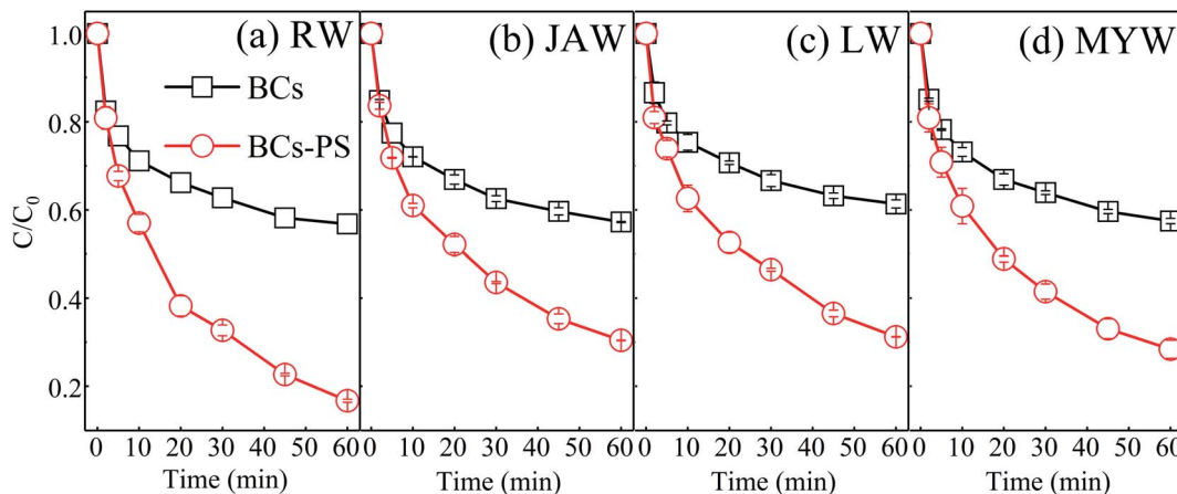
Fig. 12 BPA removal in simulated wastewaters ( [BPA]_0 = 0.02 \text{ mM} , T = 25 \pm 1 \text{ }^\circ\text{C} , [BCs]_0 = [Cs]_0 = 0.1 \text{ g L}^{-1} , [PS]_0 = 2 \text{ mM} , pH_0 = 4.0 \pm 0.1 ).
