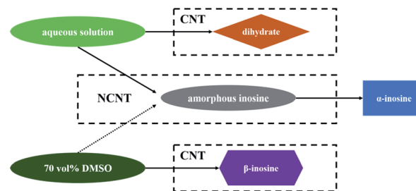
Scheme 2 Explanation for the selective crystallization from IR solutions (aqueous solution and 70 vol% DMSO aqueous solution) through MFRDS analysis. CNT refers to classical nucleation process and NCNT refers to non-classical nucleation process.
