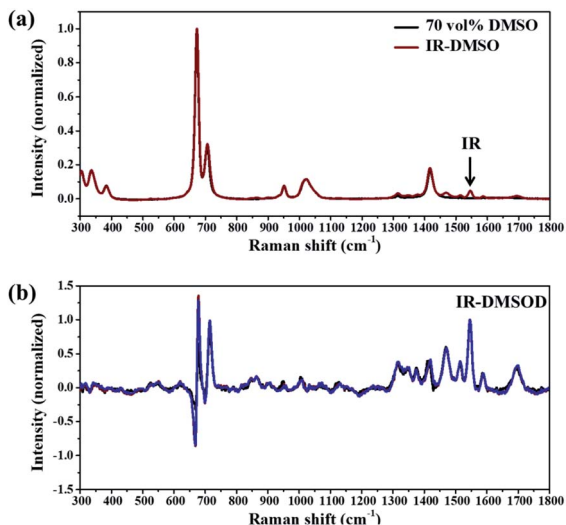
Fig. 3 MFRS of (a) 70 vol% DMSO aqueous solution (DMSO) and saturated 70 vol% DMSO aqueous solution of IR (IR-DMSO), (b) IR-DMSOD (the results of three parallel tests are shown here).
