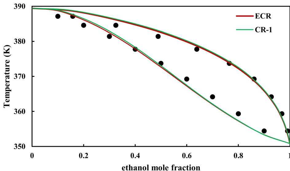
Fig. 16 T_{xy} diagram of ethanol-EDA by CPA EoS (EDA with 4C scheme) at P = 98.66 kPa, experimental data from ref. 14 (points).
