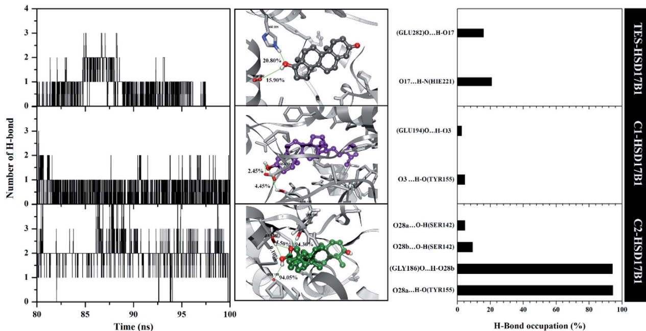
Fig. 7 Hydrogen bonding analysis: number of H-bonds (left), with a close-up of each complex in the binding pocket area (middle), and percentage of H-bonds (right). Note: cutoff value: distance <math>< 3.5 \text{ \AA}</math> and angle >math>> 120^\circ</math>.
