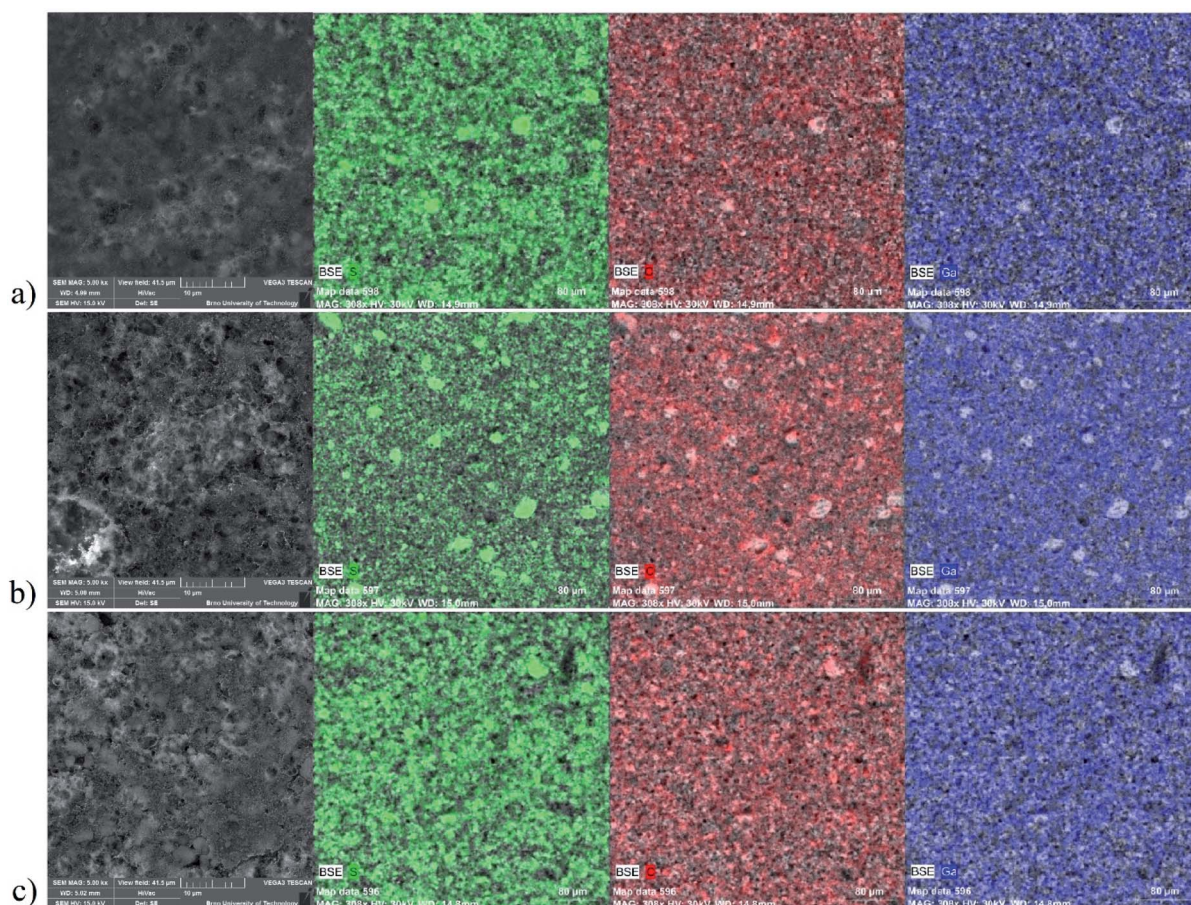
Fig. 5 SEM images and elemental mapping (S – green colour, C – red colour and Ga – blue colour) of the prepared electrode materials based on sulphur with: (a) GaTCPP(AS), (b) GaTCPP(Co) and (c) GaTCPP(Ni).
