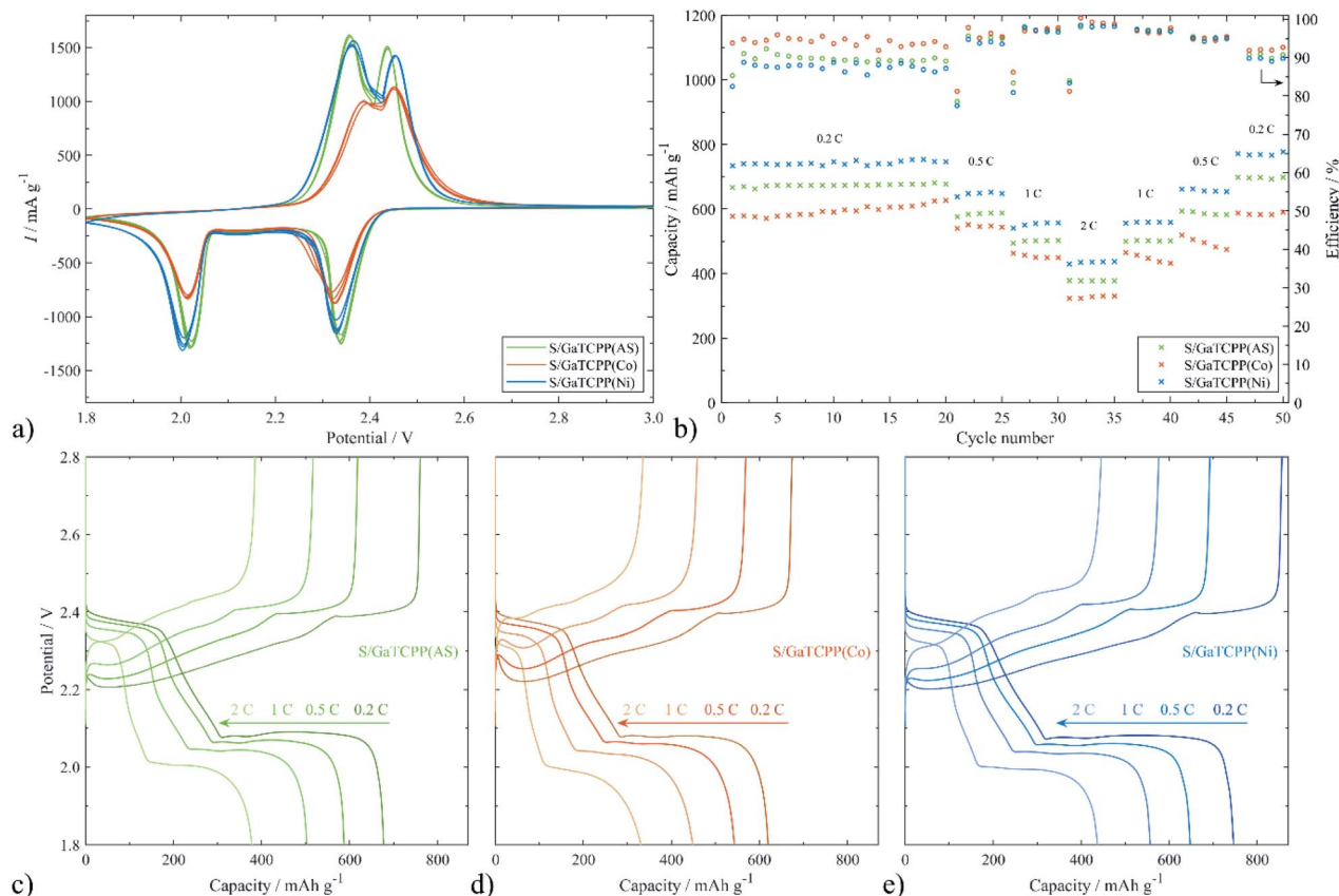
Fig. 7 Electrochemical performance of the electrodes based on GaTCCP: (a) cyclic voltammograms at a scan rate of 0.1 \text{ mV s}^{-1} ; (b) galvanostatic cycling at different C-rates; charge and discharge curves of the cell with the (c) S/GaTCCP(AS), (d) S/GaTCCP(Co) and (e) S/GaTCCP(Ni) cathode.
