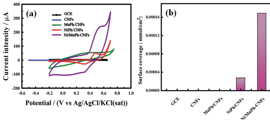
Fig. 7 (a) CVs responses for different electrodes GCE, CNFs, MnPh/CNFs, NiPh/CNFs, NiPh/MnPh-CNFs at 50 \text{ mV s}^{-1} scan rate. (b) Bar chart of the surface coverage ( \Gamma ) values of different electrode materials GCE, CNFs, MnPh/CNFs, NiPh/CNFs, Ni/MnPh-CNFs.
