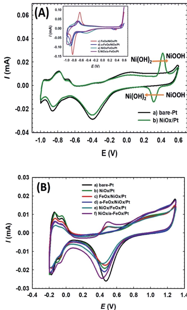
Fig. 2 CVs obtained in 0.5 mol L -1 NaOH (A) and in 0.5 mol L -1 H 2 SO 4 (B) for: (a) bare-Pt, (b) NiOx/Pt, (c) FeOx/NiOx/Pt, (d) a-FeOx/NiOx/Pt, (e) NiOx/FeOx/Pt and (f) NiOx/a-FeOx/Pt catalysts at a scan rate of 200 mV s -1 .
