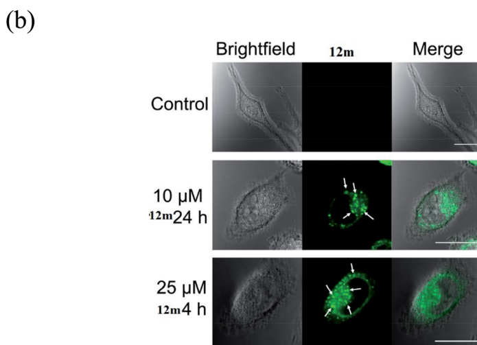
Fig. 2 (a) Structures of fac-[Re(CO) 3 (N-N)(OH 2 )] + complexes. (b) Brightfield and confocal fluorescent microscope images of control HeLa cells and HeLa cells treated with 12m. Arrows point to vacuoles induced by 12m treatment. Scale bars = 20 \mu m. [Adapted from ref. 26 with permission from the American Chemical Society].
